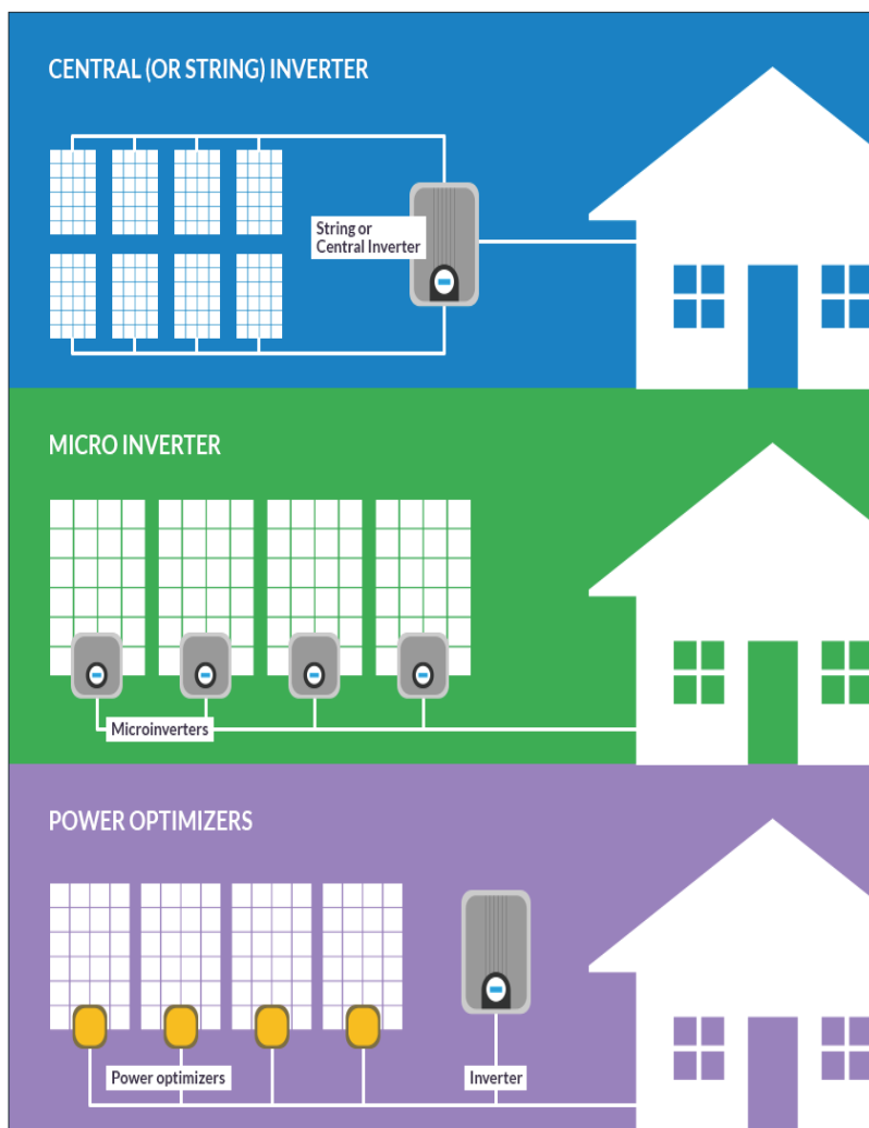
Figure 2: Types of Inverters
