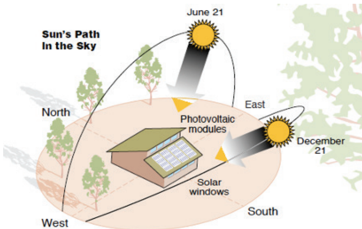
Figure 7: The Path of the Sun in New England
